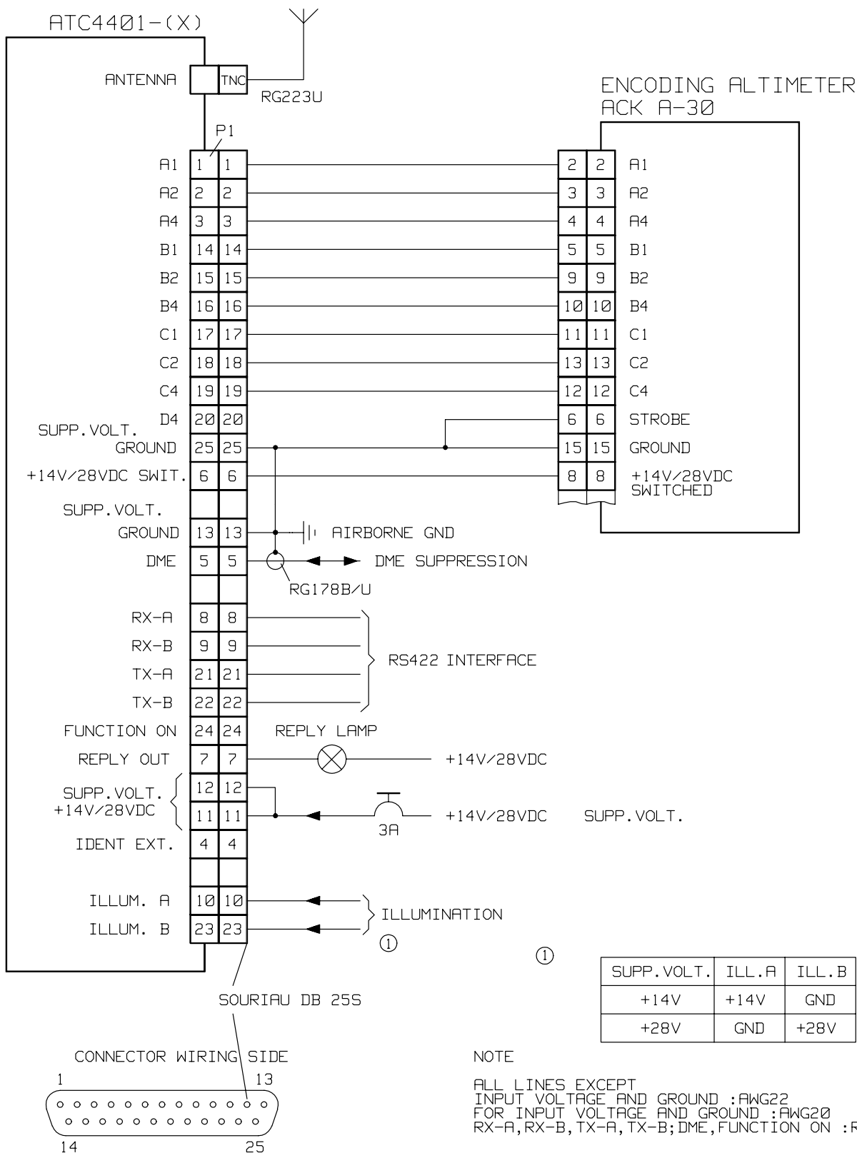
Fig. 2-4 Installation wiring ATC 4401-(x) with encoding altimeter ACK A-30 (PRELIMINARY)
